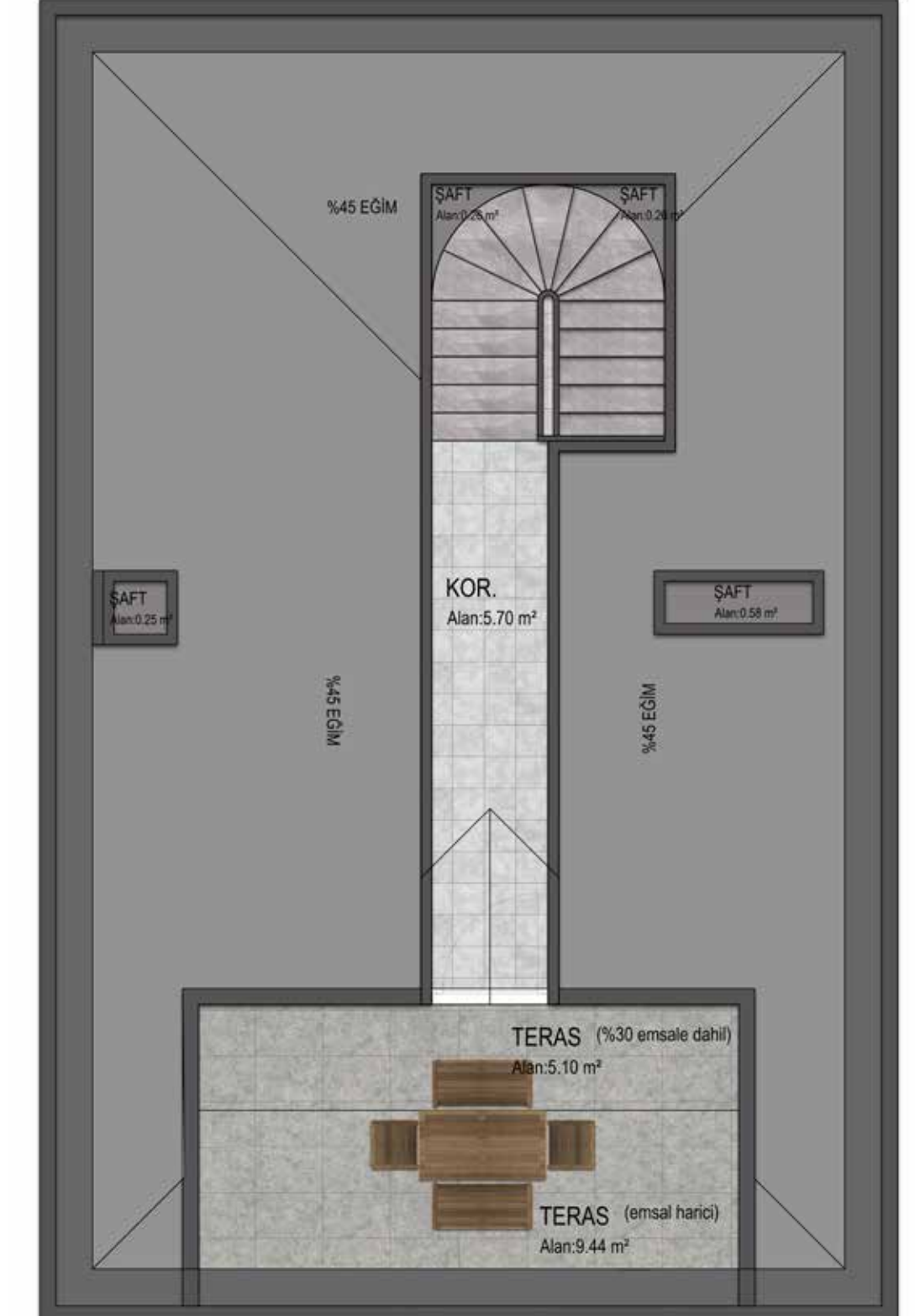
ÇATI KAT PLANI
